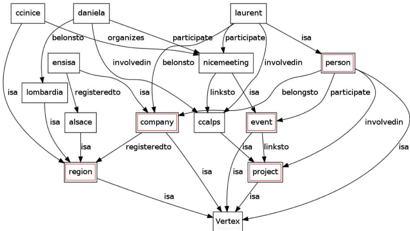
Figure 8. Partial model &amp; metamodel behind CCAIps
