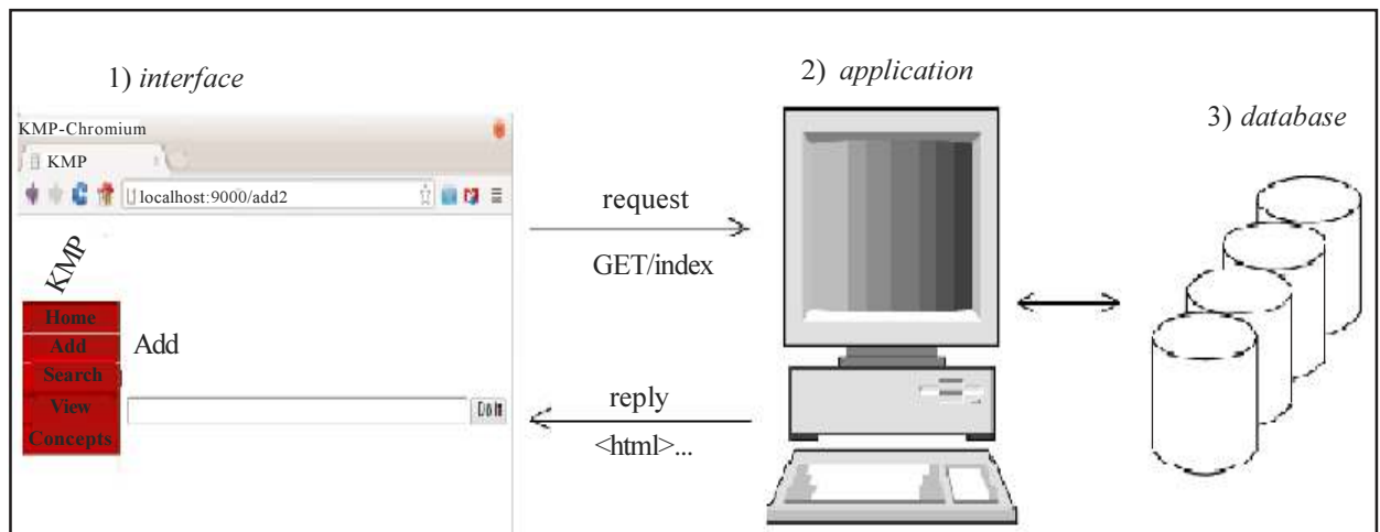
Figure 4. 3-layers architecture
