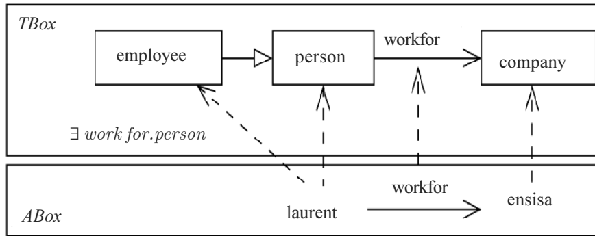
Figure 3. Separation TBox/ABox
